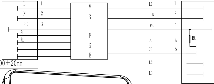
Connection Diagram
