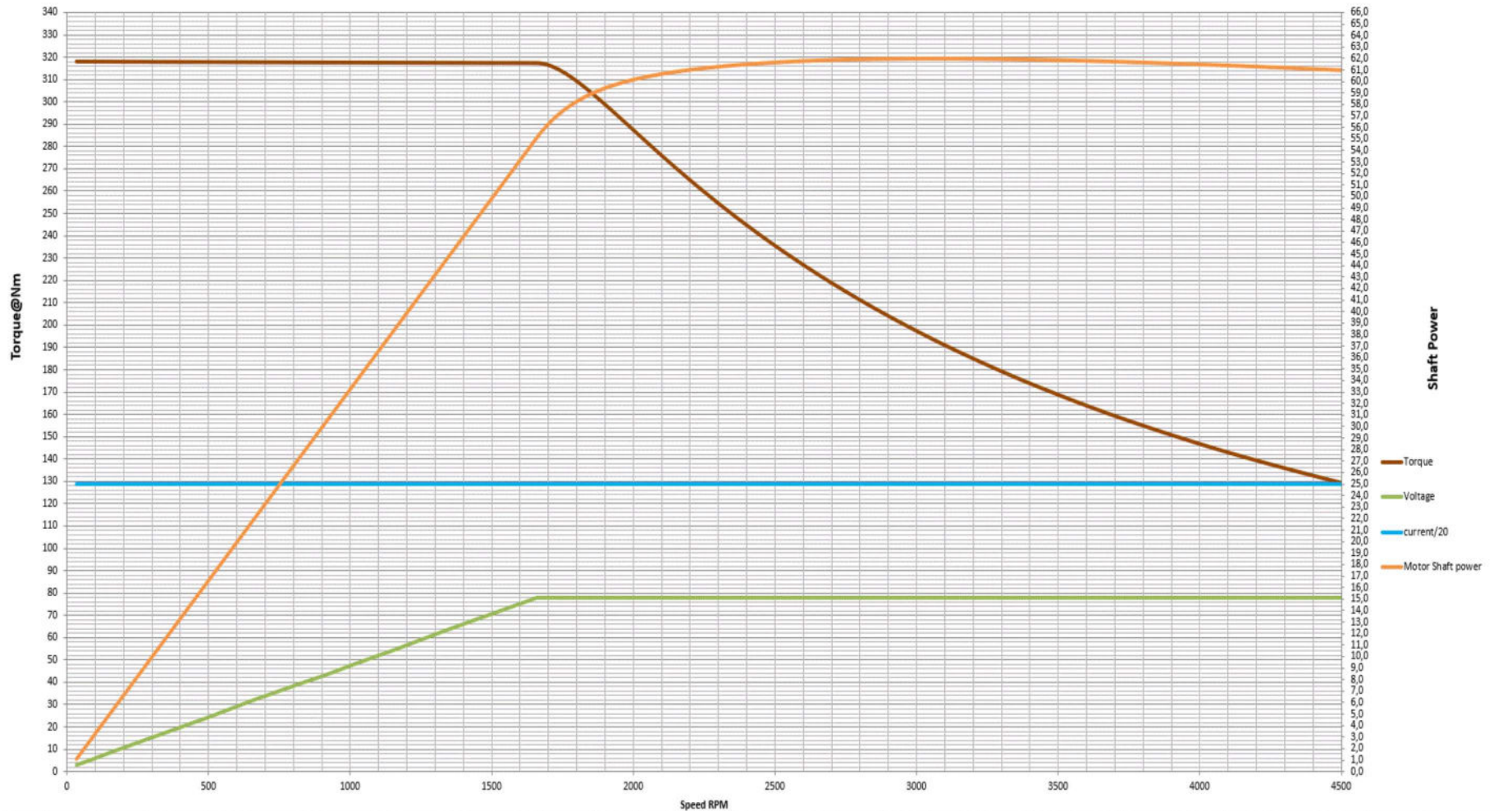
Torque Curve
